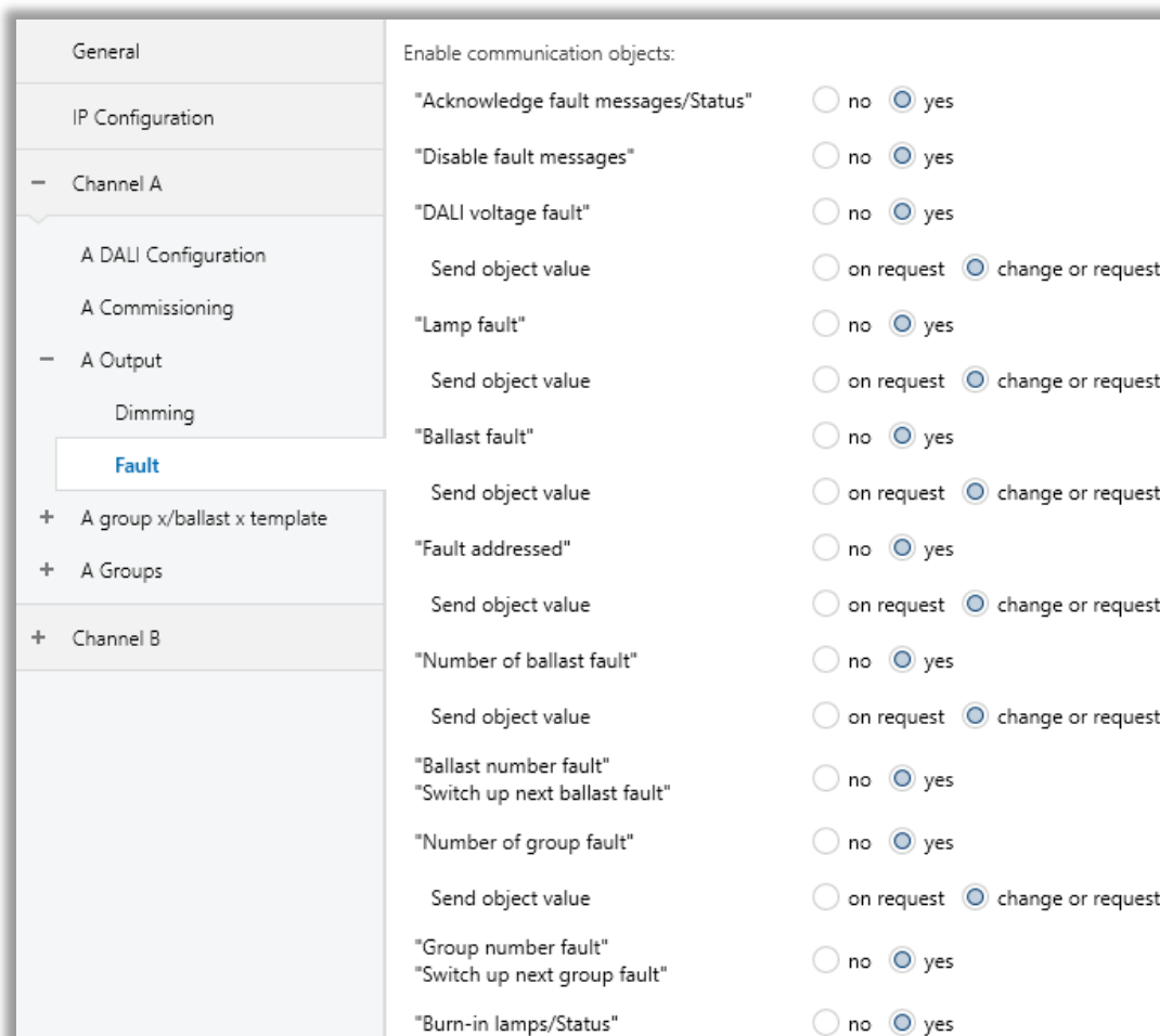
Fig. 13: Fault Function Configuration
