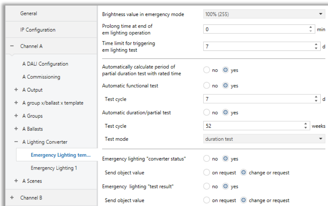
Fig. 28: A Lighting Converter – Emergency Lighting Template Configuration
